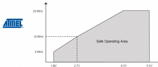
Figure 28-1. Maximum Frequency vs. V_{CC}
